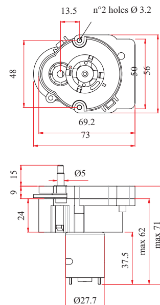
SERIES 262 WITH CAM & MICROSWITCH 24V DC
