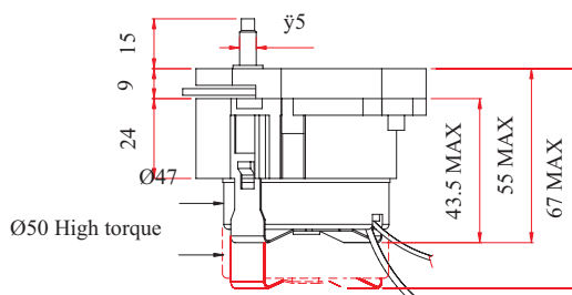
SERIES 262 WITH CAM & MICROSWITCH 24/117/230V AC
